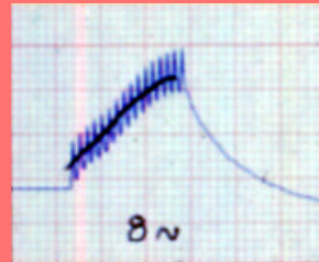
Weld 8 Cycles
