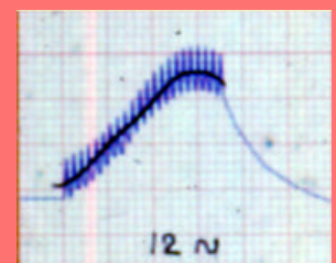
Weld 12 Cycles
