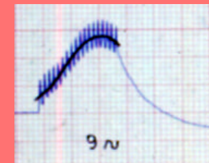
Weld 9 Cycles
